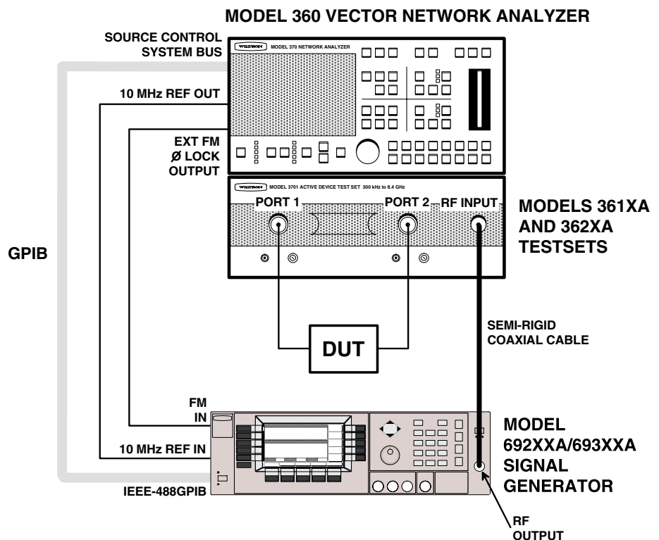
Figure 7-3. 692XXA/693XXA to 360B VNA Connections
