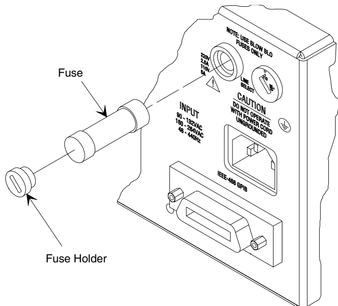
Figure 6-1. Replacing the Line Fuse
