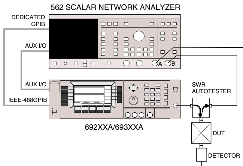
Figure 7-2. 692XXA/693XXA to 562 SNA Connections
